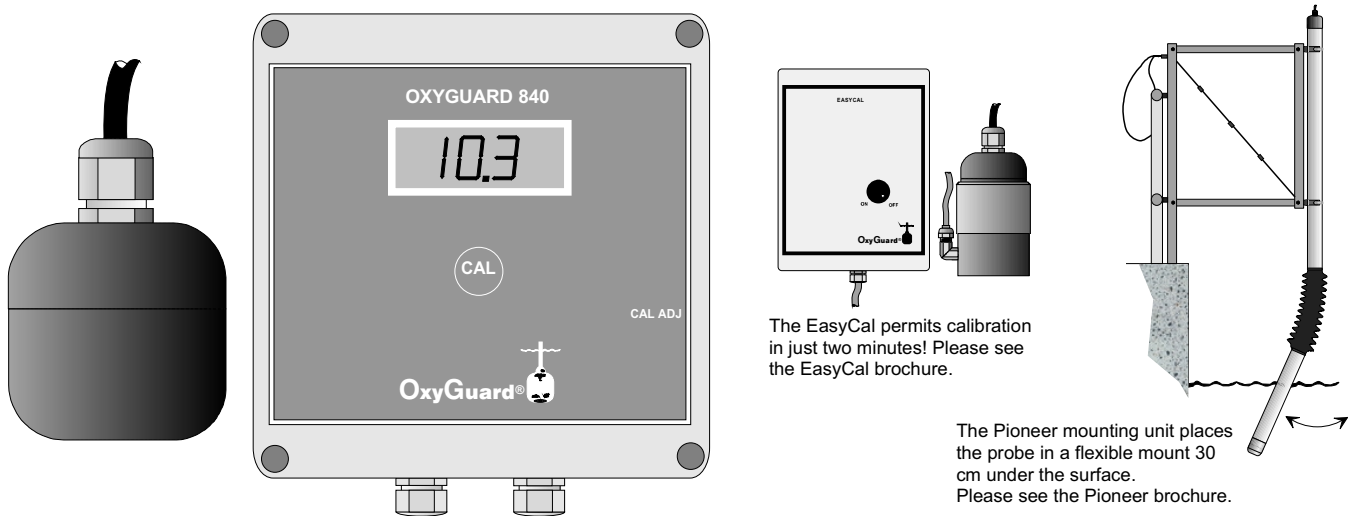
840 Probe and Display Box shown half size
