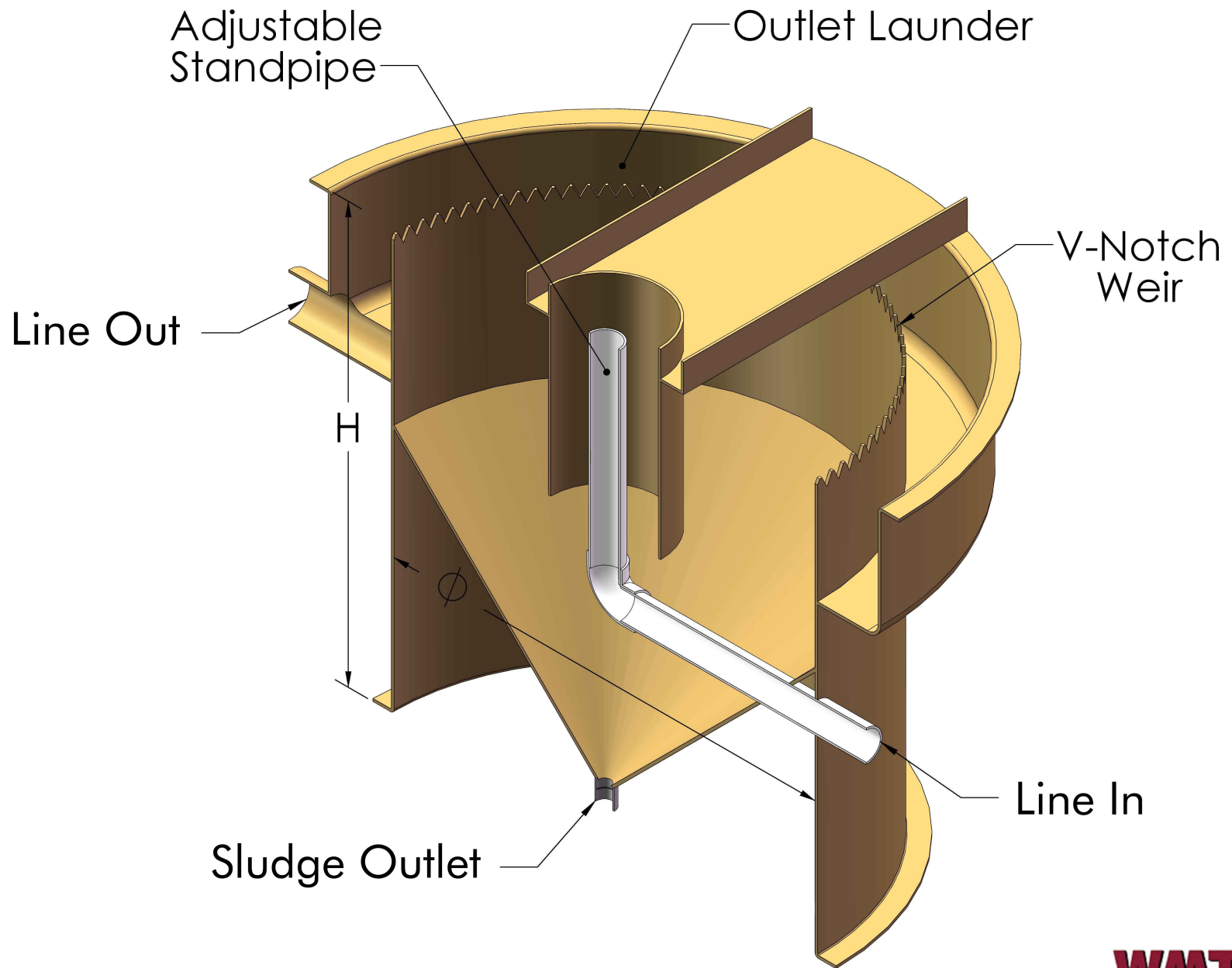
Radial Flow Separator (RFS)
