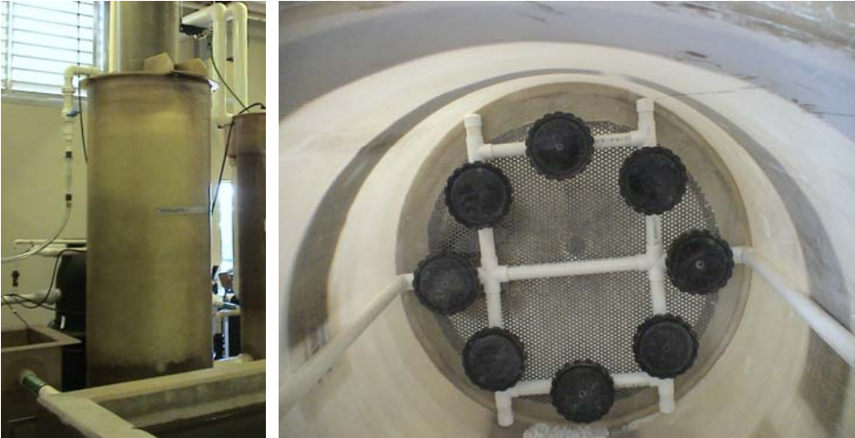
Go Fish GA – Vertical IMF Biofilter with Air Grid and Media Screen – 6 systems (60-180 gpm), 15-75 ft 3 media (0.42-2.1m 3 )
